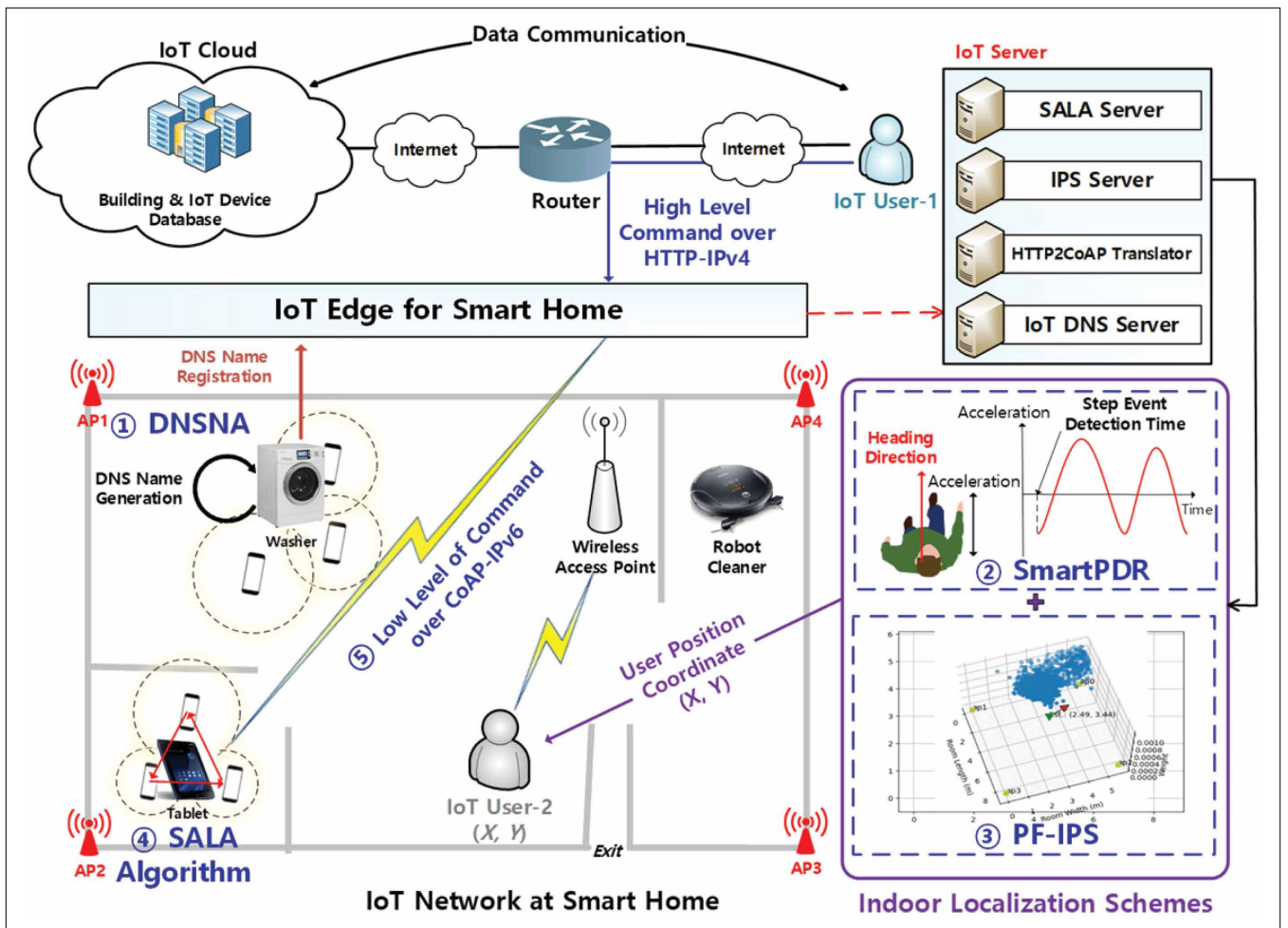
FIGURE 1. The workflow of the IoT Edge-Cloud system.
