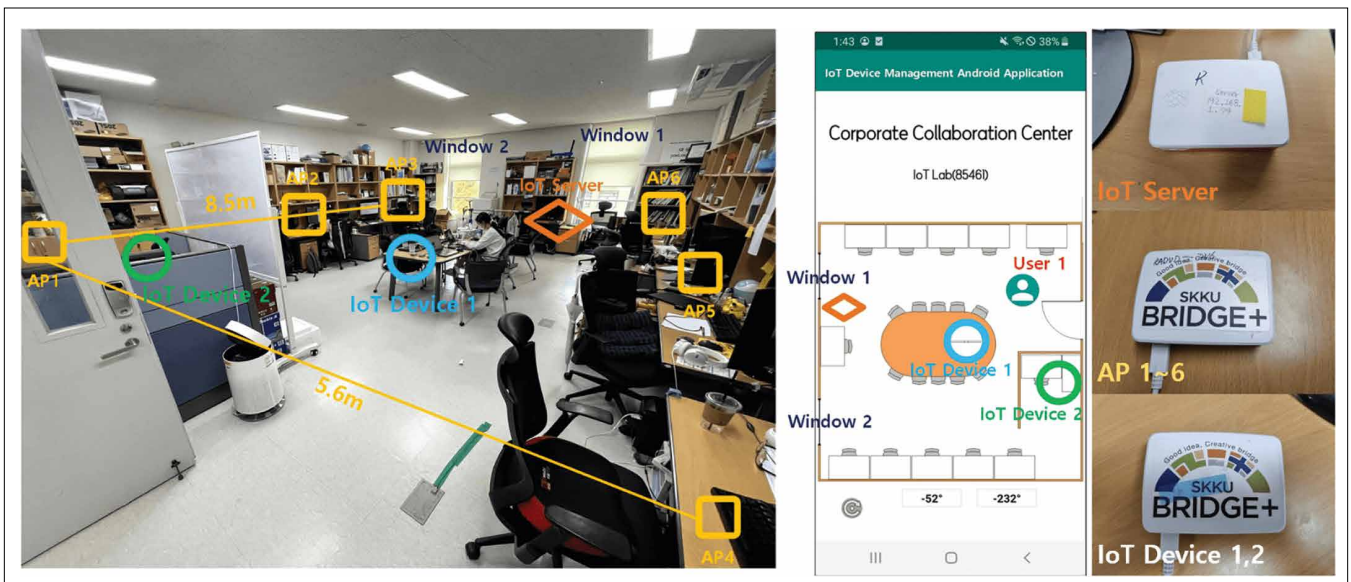
FIGURE 3. Testbed and smartphone App for IoT device localization.
