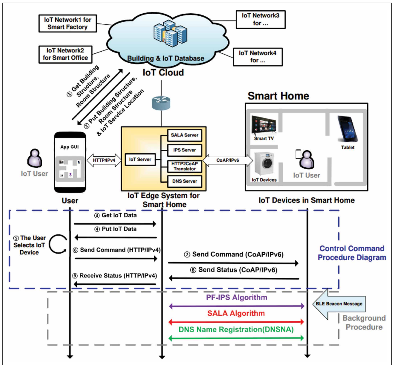
FIGURE 2. The sequence diagram of the IoT Edge-Cloud system.
