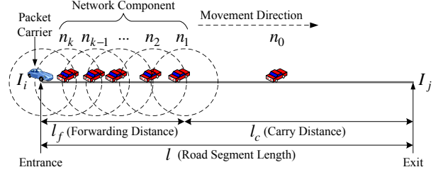
Figure 1. Forwarding Distance l_f and Carry Distance l_c
