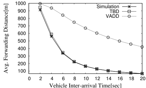
Figure 3. Validation and Comparison of Analytical Models
