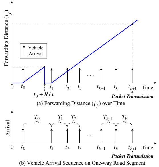
Figure 2. Forwarding Distance ( l_f ) for Vehicle Arrivals
